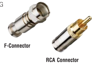
RCA Connector
